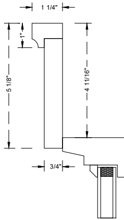
Brickmold Casing
