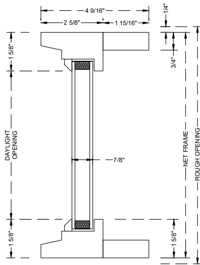
Head & Sill
