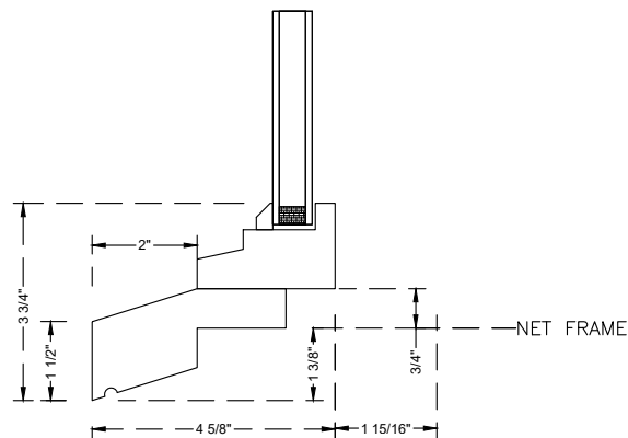
True Subsill (2816)
