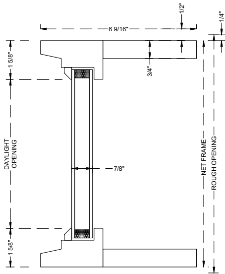
Head & Sill
