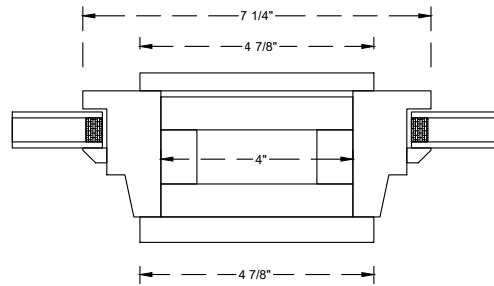
4" Spread Mull
