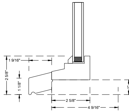
Subsill (2814)
