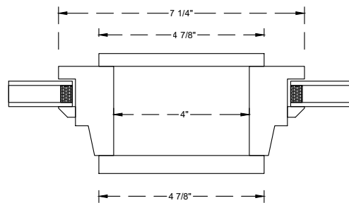
4" Space Mull
